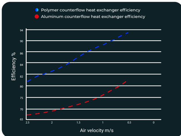
Dependence of efficiency on airflow velocity for counterflow heat exchangers.
